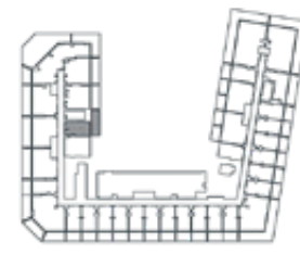
STUDIO TYPE 02
